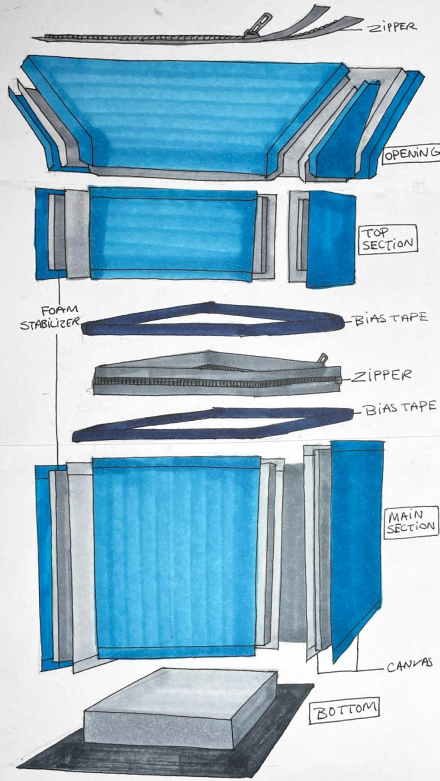
EXPLODED VIEW - BACKPACK
